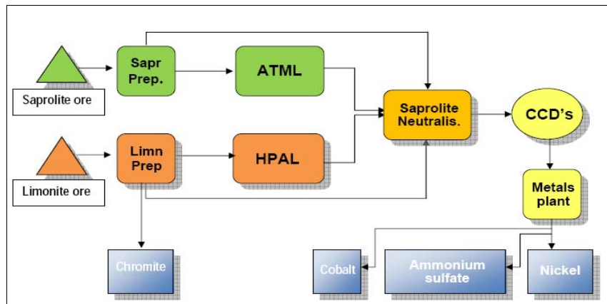
Fig. 1. Simplified flow sheet for the Mindoro Nickel laterite processing
